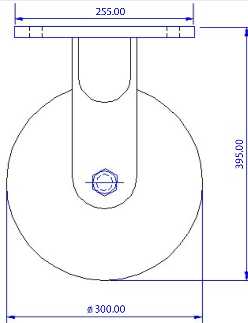
FRONT VIEW
