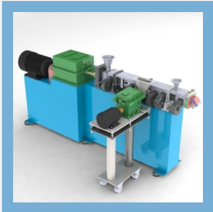
Twin Screw Extruder
