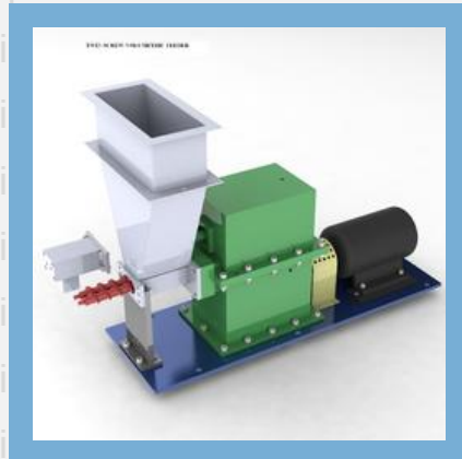
Twin Screw Volumetric Feeder
