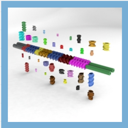
Twin Screw Shaft
