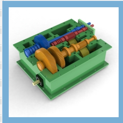
Twin Screw Co-rotating Gear Box
